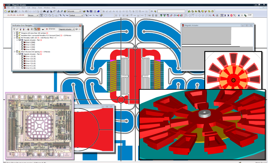
A central part of the MEMS design flow, here L-Edit MEMS is shown being used to design a magnetic actuator; the tool allows for the quick creation of entire complex curved shapes for MEMS from just a few easily drawn shapes.
